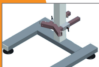
Belt clamping system 12-1038
